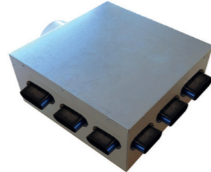
2 Plénum 9 piquages extraction / insufflation Raccord Ø 125 mm 150/160 mm PLI 50/5P 810 509
