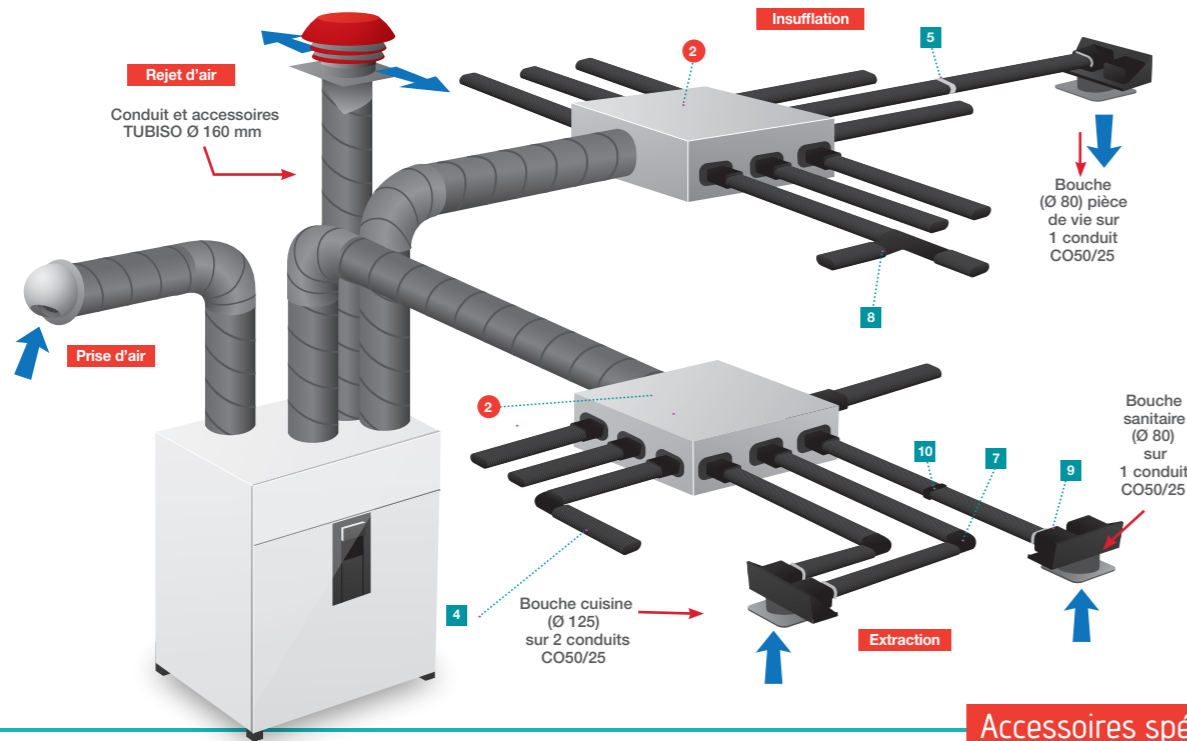
2 Plénum 9 piquages extraction / insufflation Raccord Ø 125 mm 150/160 mm PLI 50/5P 810 509
